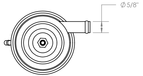
W-4000-C AIR SEP ASSY W-4026 CAN TOP W-4015 CAN BOTTOM
